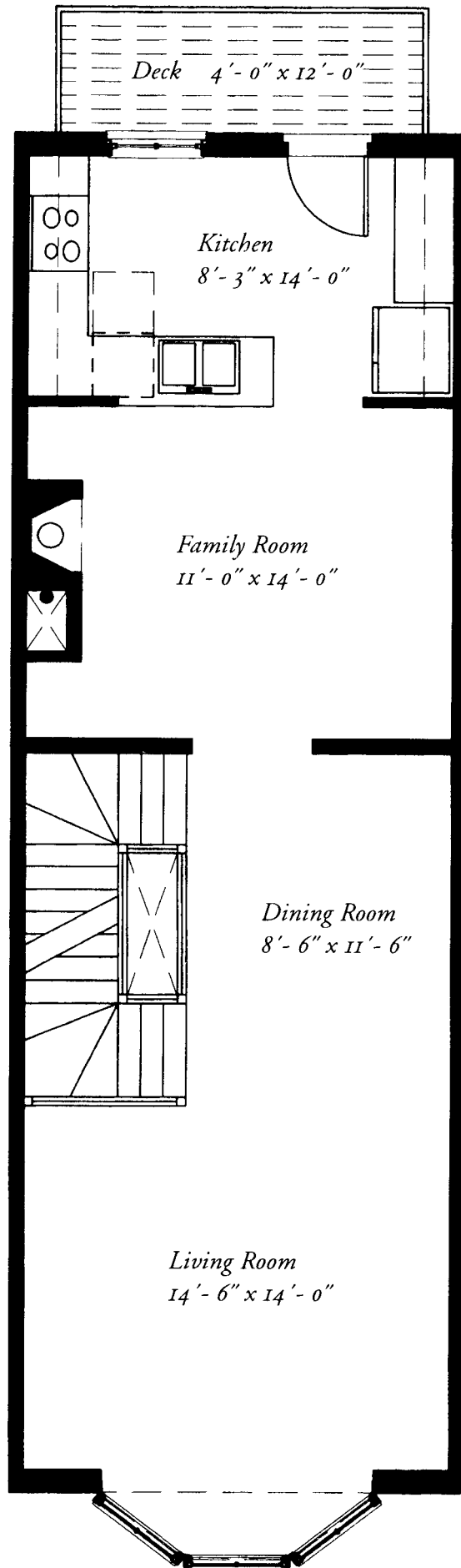
First Floor ( 11-foot ceiling )
